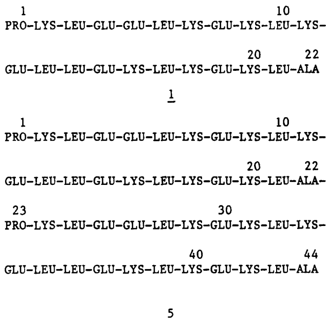
Figure 3. Amino acid sequences of peptides 1 and 5, models for apolipoprotein A-I.
